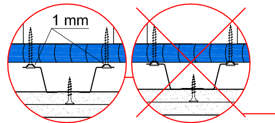
Image 23: Method of resilient ceiling connection via flexible hanging steel profile
