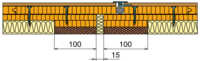
Image 27: Floor dilatation for example at doors to the rooms.
