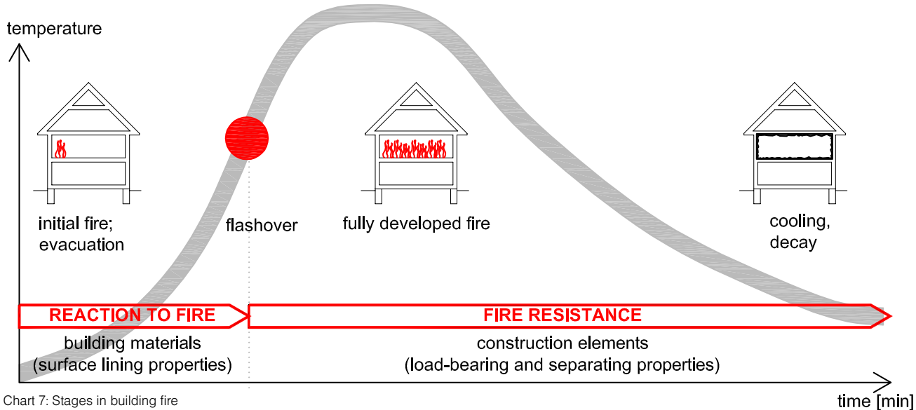
Chart 7: Stages in building fire
