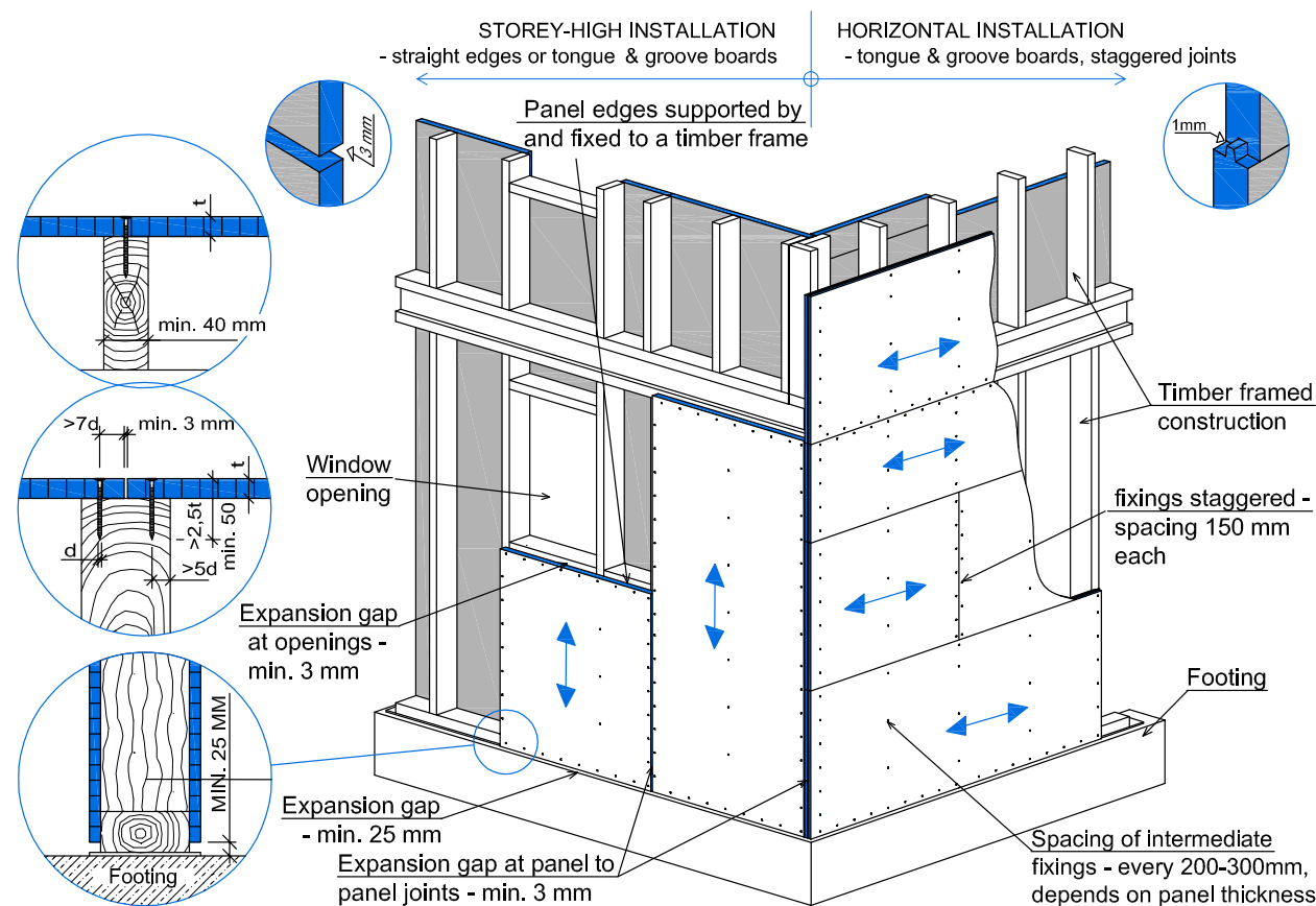
Image. Wall installation form boards vertically on the pillars
