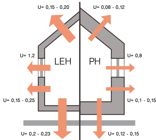
Image 3: Schematic visualization of different requirements for heat transfer coefficient U for various constructions between low-energy (LEH) and passive houses (PH).
