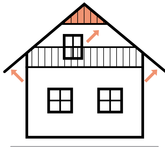
Image 16: Roof covering. In this case the protected exterior is under wood as a condition of use in moisture class 2.
