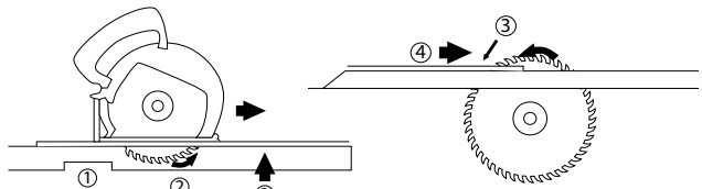
Image 5 - Hand-held circular saw cutting:
