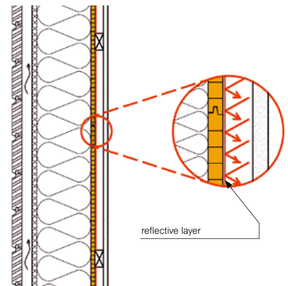
Image 8. High reflectivity – prevention of heat losses
