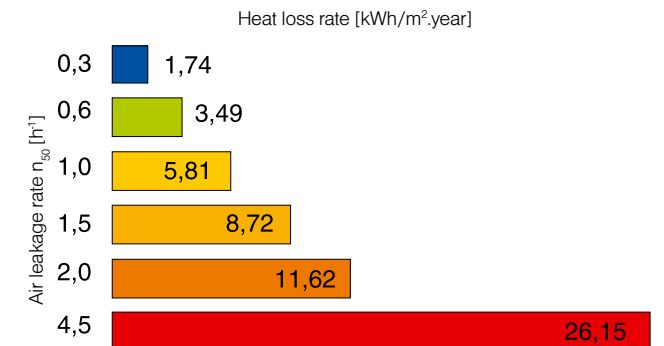
Chart 3: Increased air permeability of building constructions has resulted in an increase of heat loss rate and thus the energy needed for heating. For ordinary buildings with conventional ventilation ( n_{50} = 4.5 \text{ h}^{-1} ) are the heat losses due to increased air permeability of the envelope nearly eight times higher than for passive houses with a value of n_{50} = 0.6 \text{ h}^{-1} . (see Figure 1) .
