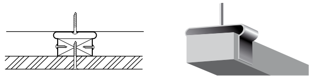
Image 21: Spring clamps for fixing beams with exterior cladding to the load-bearing construction.
